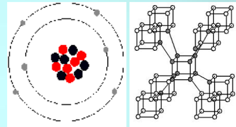
Atomic Structure of C
